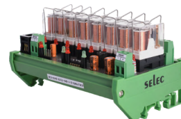
ERLYMD-2-1-S8-1CO-24V 87(H) x 138(W)mm
